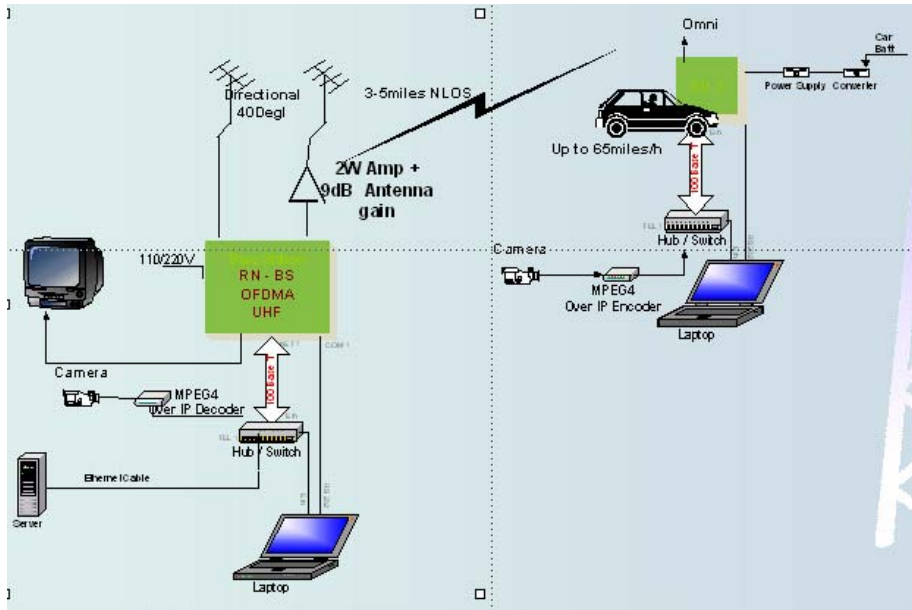
Mobile video surveillance in UHF band
