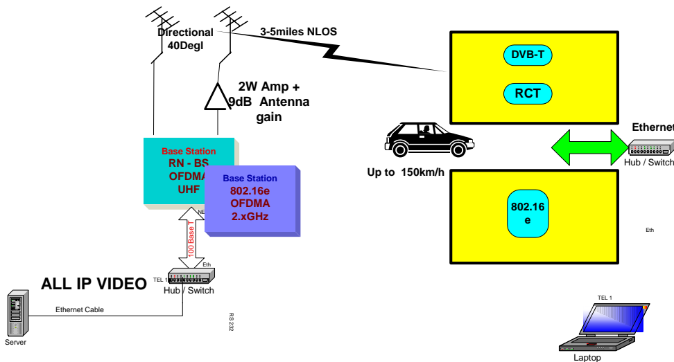
Test scenario 1 in both UHF and 2.3GHz band
